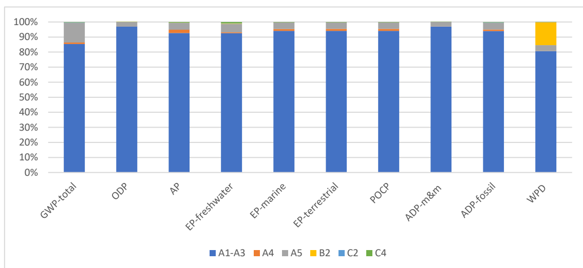
Figure 2 Environmental profile of 1 m 2 of ceramic tiles (Group BIII)
